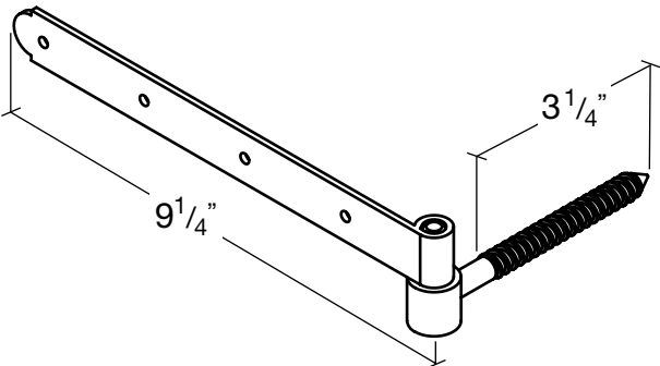
New York Strap Hinge Set - Lag Mount
