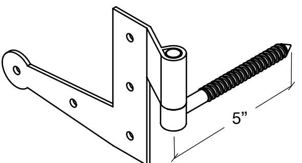
Suffolk 'L' Hinge Set - Lag Mount
