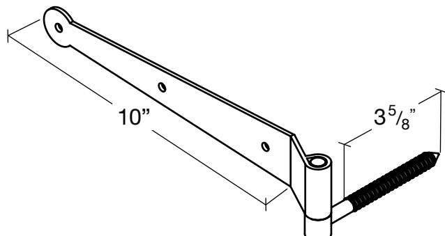
Suffolk Strap Hinge Set - Lag Mount
