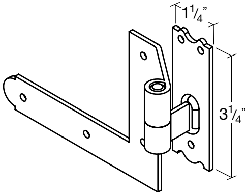
New York 'L' Hinge Set - Plate Mount
