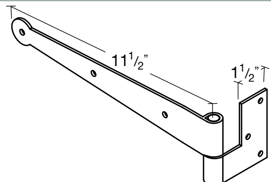
Suffolk Strap Hinge Set - Jamb Mount
