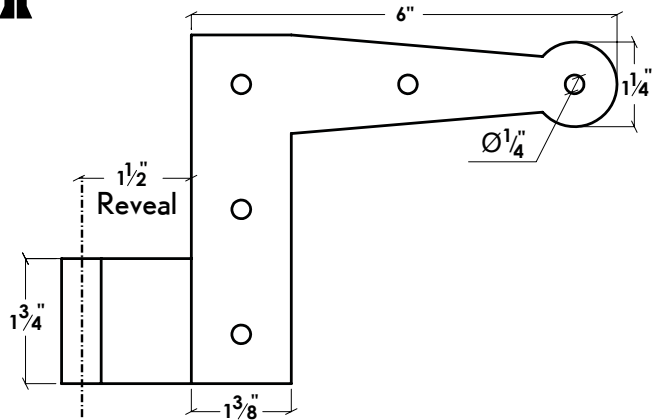
Suffolk 'L' Hinge
