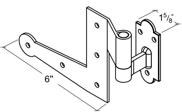
Surface Mount
