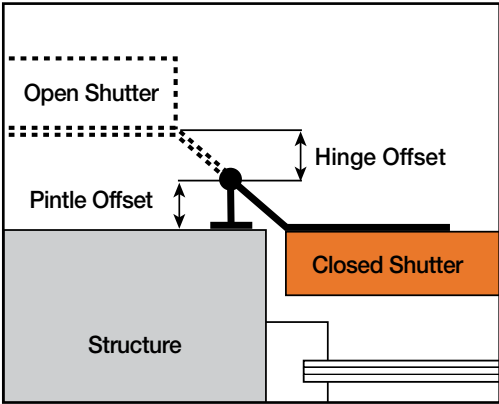
Flush Mount
