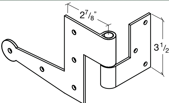
Suffolk 'L' Hinge Set - Jamb Mount
